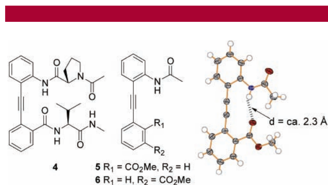
Figure 1. Model compound 5 and control isomer 6 . X-ray structure of 5 shows the hydrogen bonding interaction between adjacent units.
