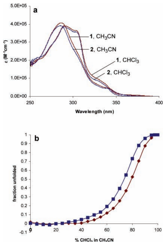
Figure 2. (a) UV spectra of 1 (red) and 2 (blue) in chloroform and acetonitrile. (b) UV titration curve of 1 (red diamonds) and 2 (blue squares).
